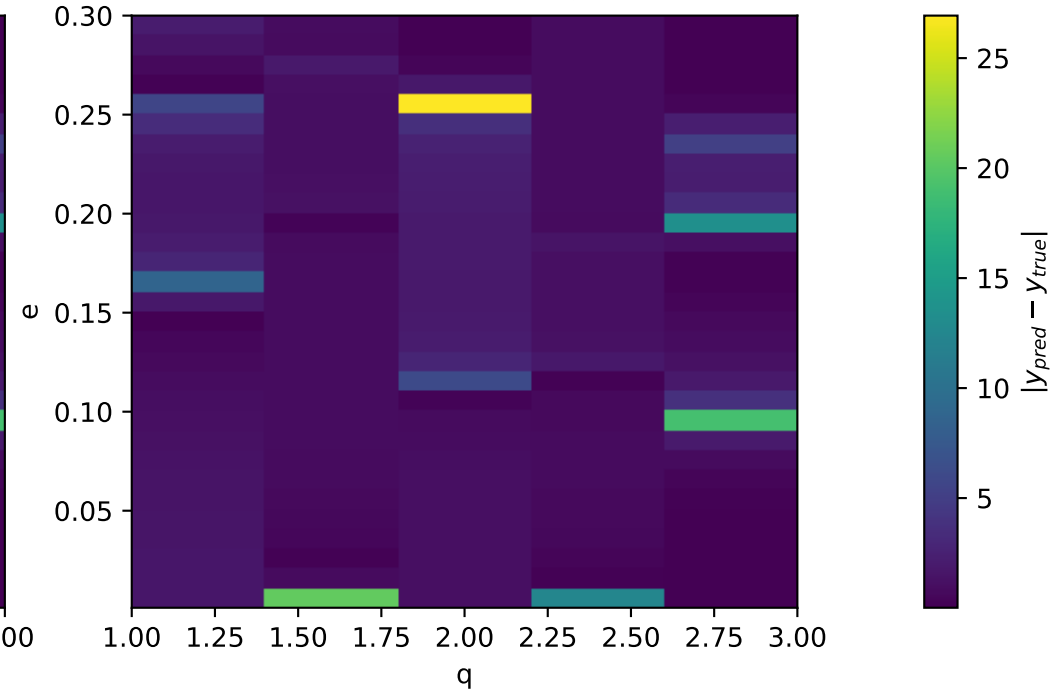
k=Aniso \nu=4.0
